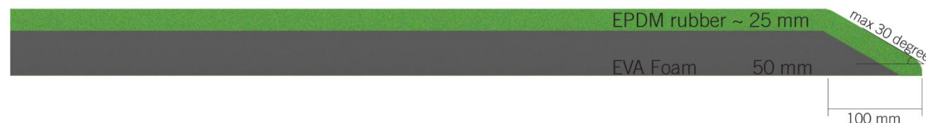
Type 3 Detail view of the Floor with 50 mm shock absorbing
